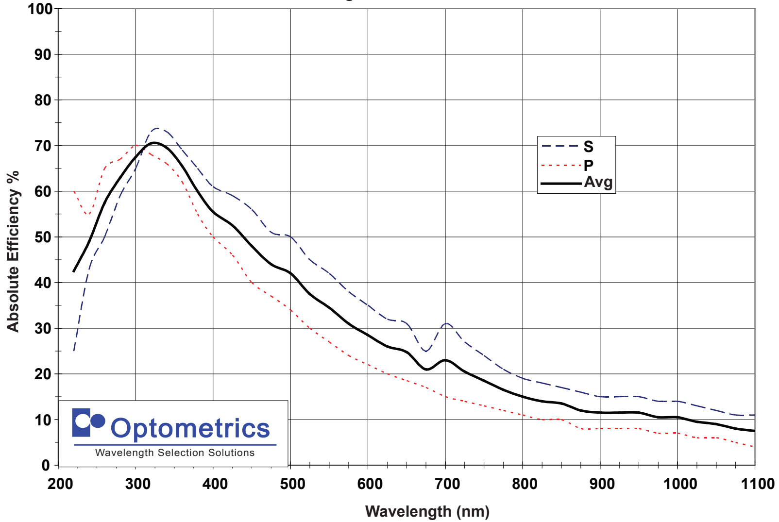
600g/mm Ruled 300 nm Blaze
