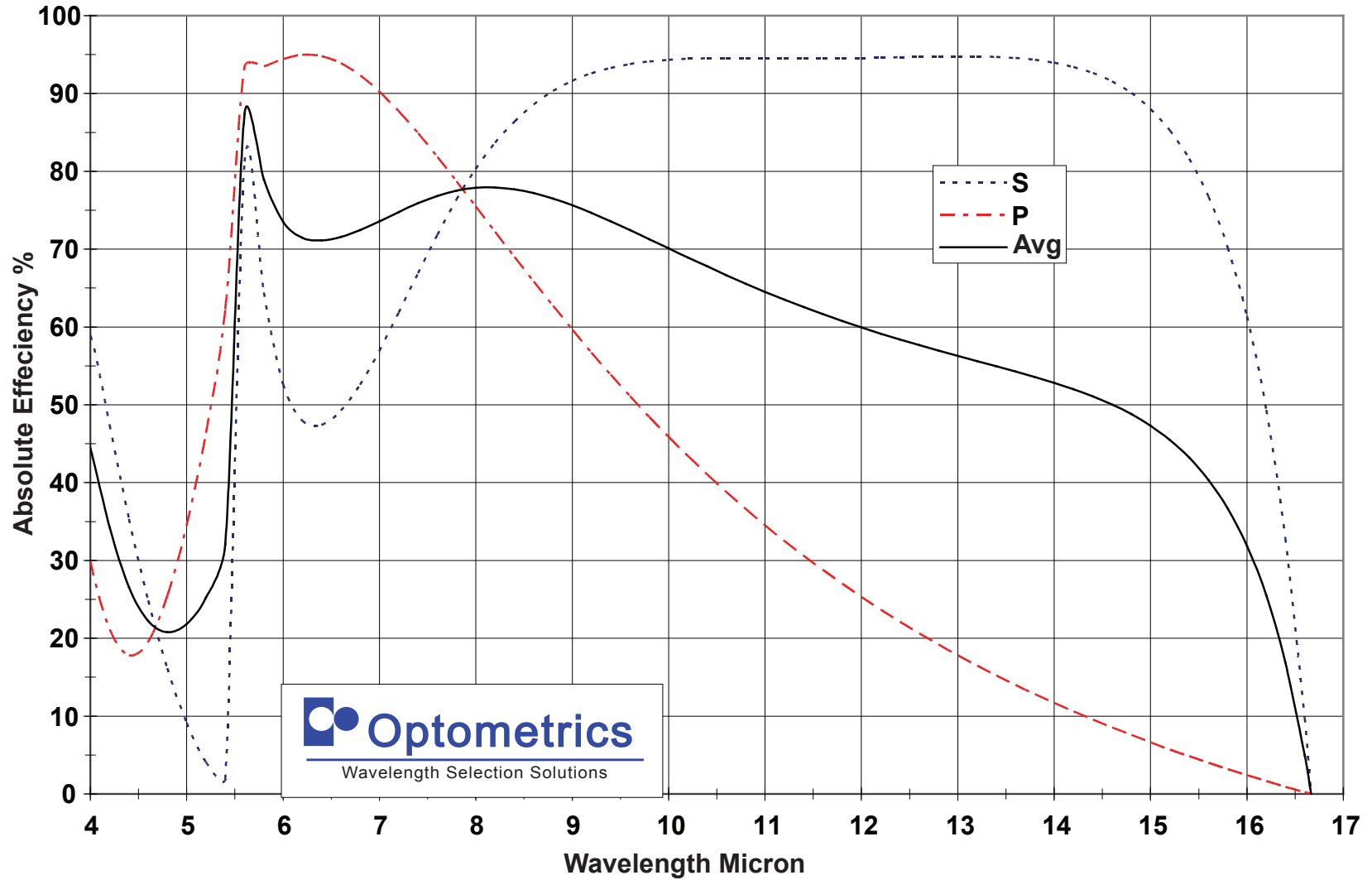
120g/mm Ruled 1.2 Micron Blaze
