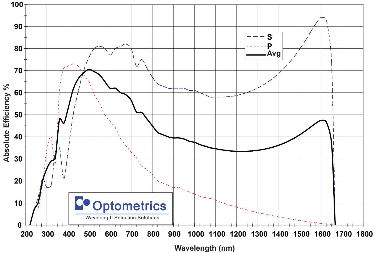
1200g/mm Ruled 500 nm Blaze
